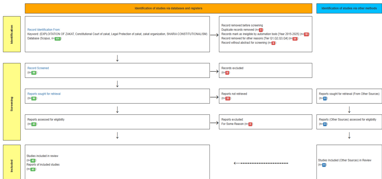
Figure 1. PRISMA Flowchart
